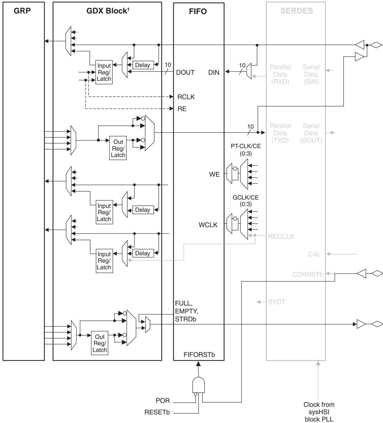
Figure 12. Operation in FIFO Mode 2
