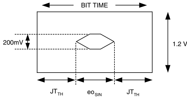
Figure 20. Receive Data Eye Diagram Template (Differential)
